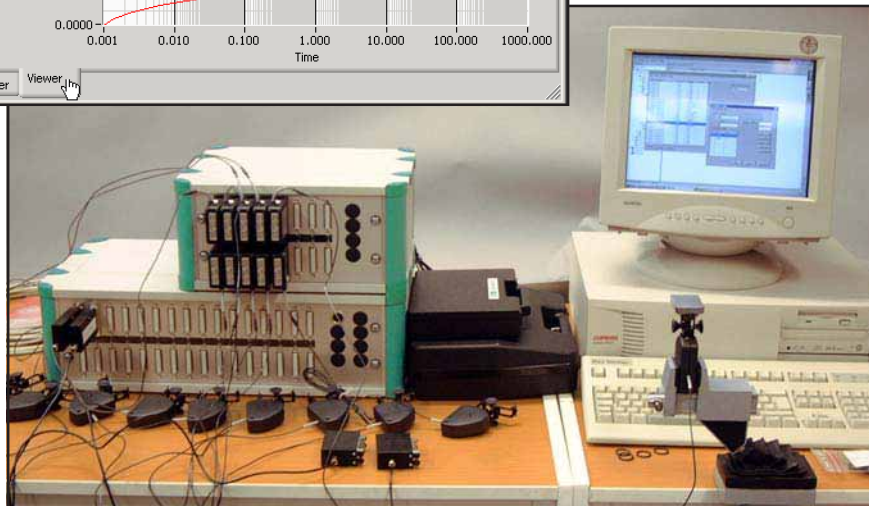
Data acquisition system for Creep tests, ED 03 C
